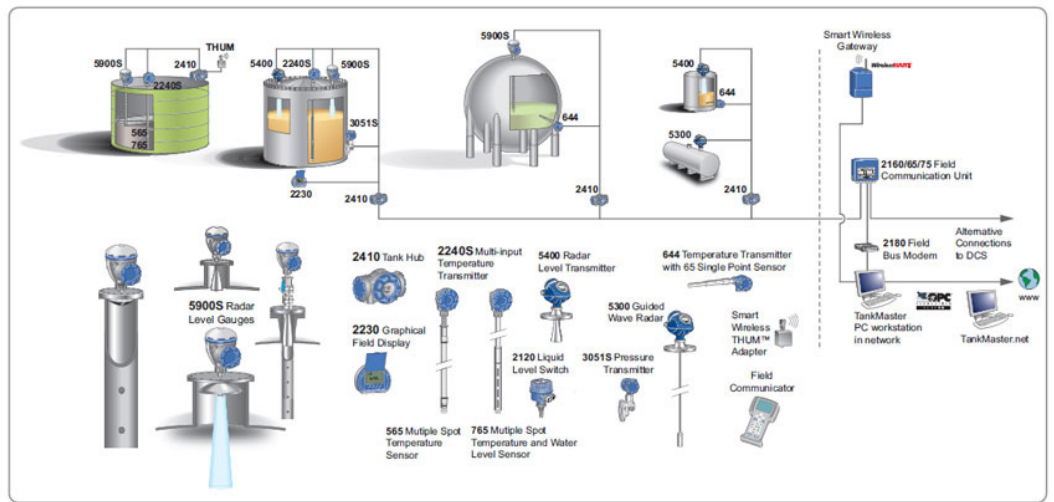
Wireless Rosemount Tank Gauging System
